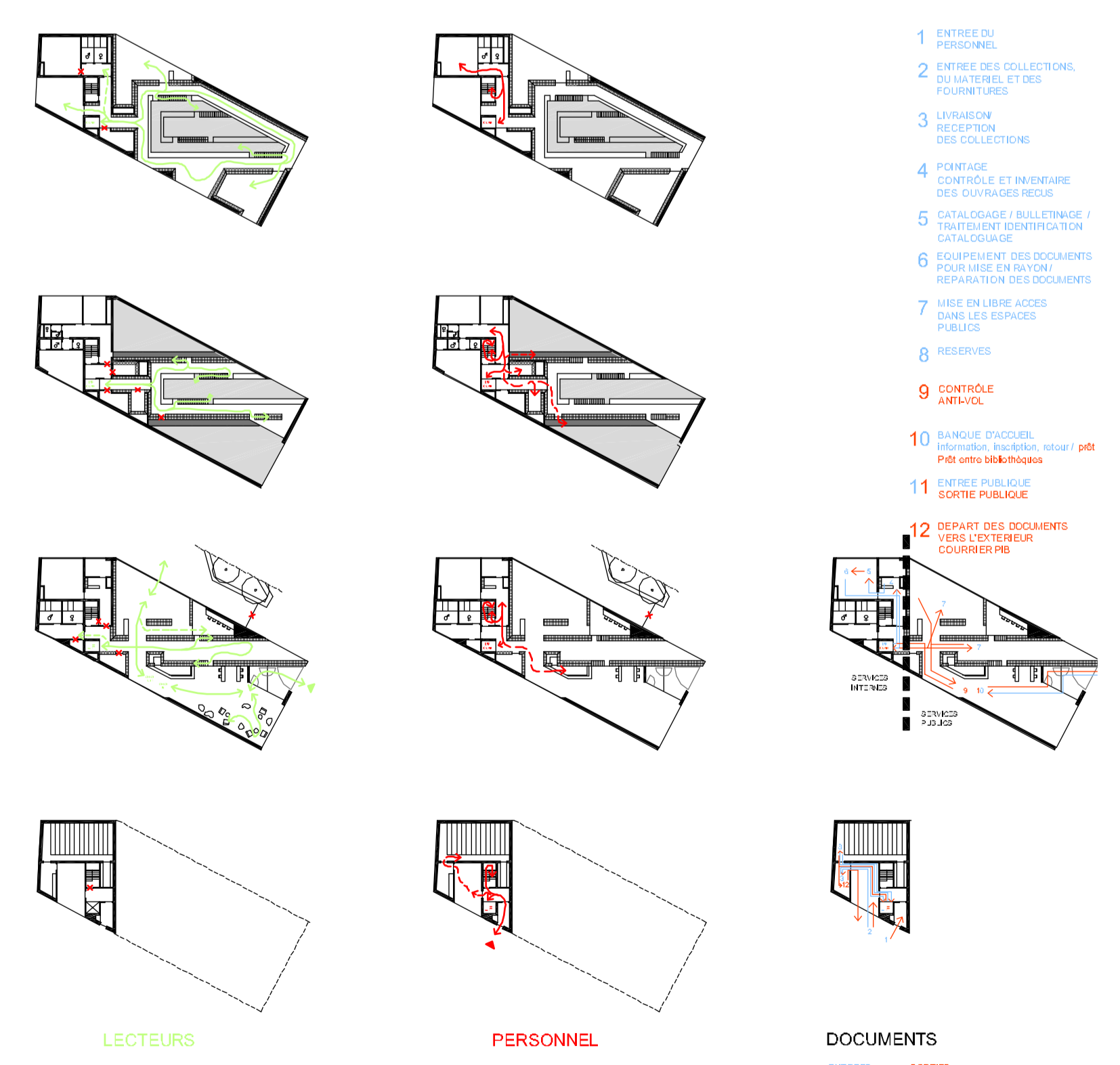
SCHEMAS CIRCULATION
