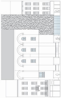
FACADE RUE BORROYAL
